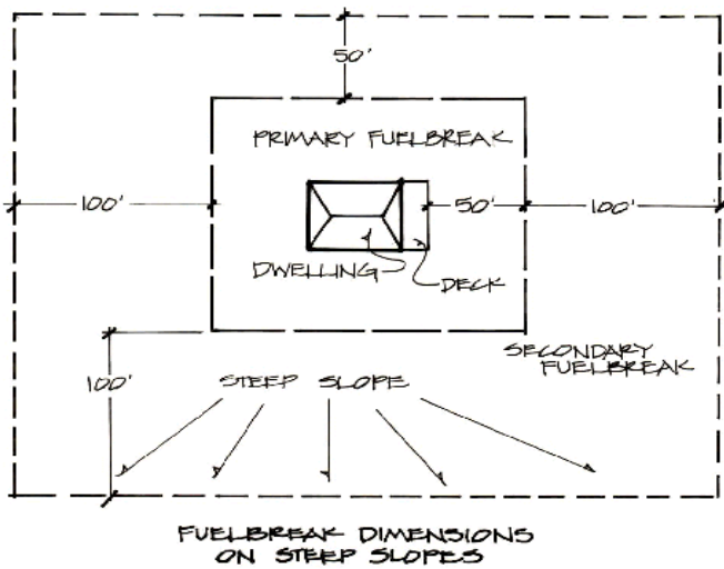
FUELBREAKS ON STEEP SLOPES
